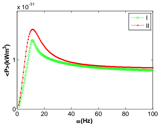
Fig. 3. Intensity of the power production vs. the field frequency \omega of the magnetic field for H_0 , in I= 4 \cdot 10^2 \text{ kA/m} and II= 5 \cdot 10^2 \text{ kA/m}
